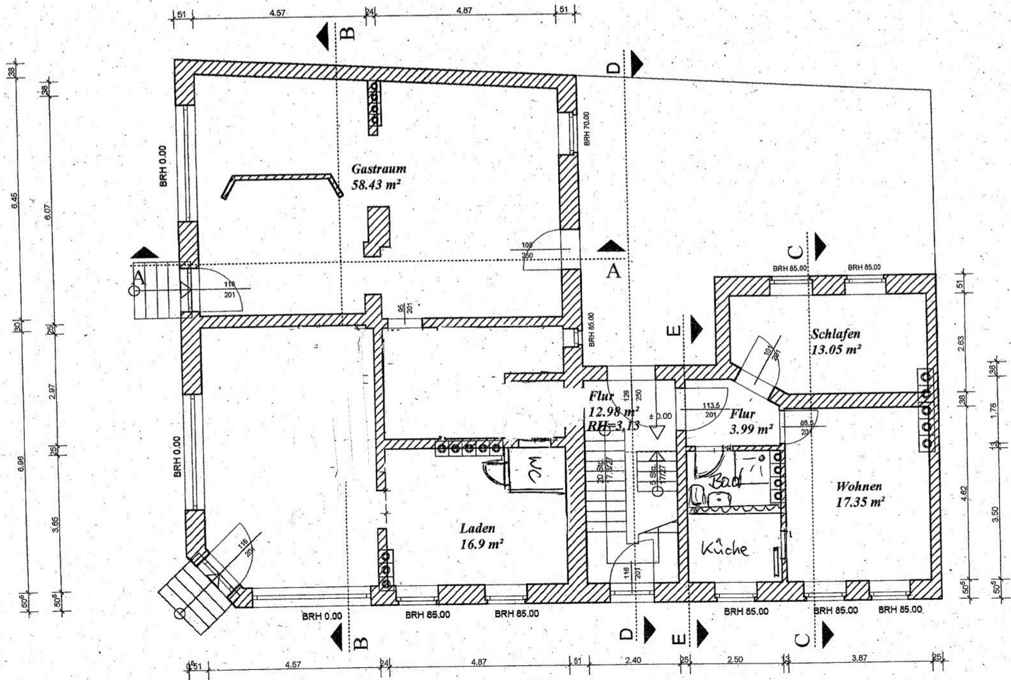
Grundriß Erdgeschoß
