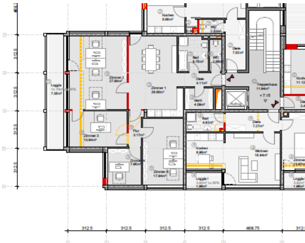
Grundriss Whg.3
