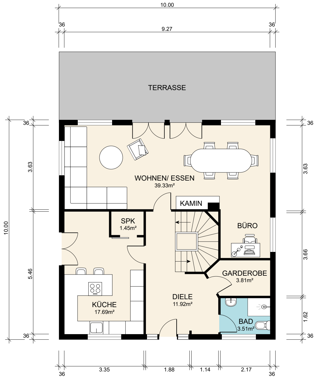
ERDGESCHOSS VERSION 1
