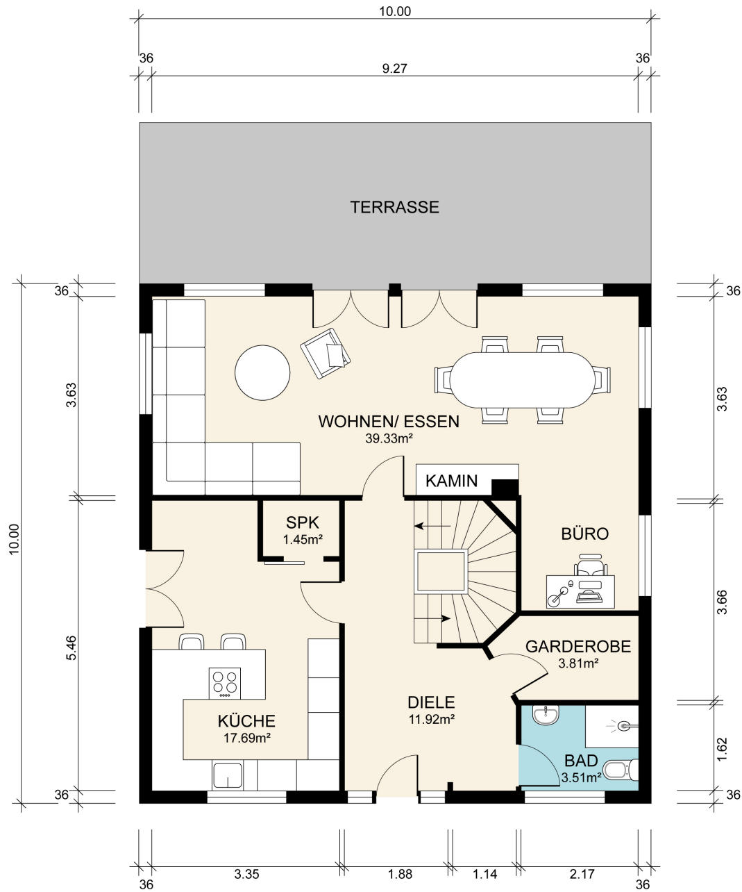
ERDGESCHOSS VERSION 1
