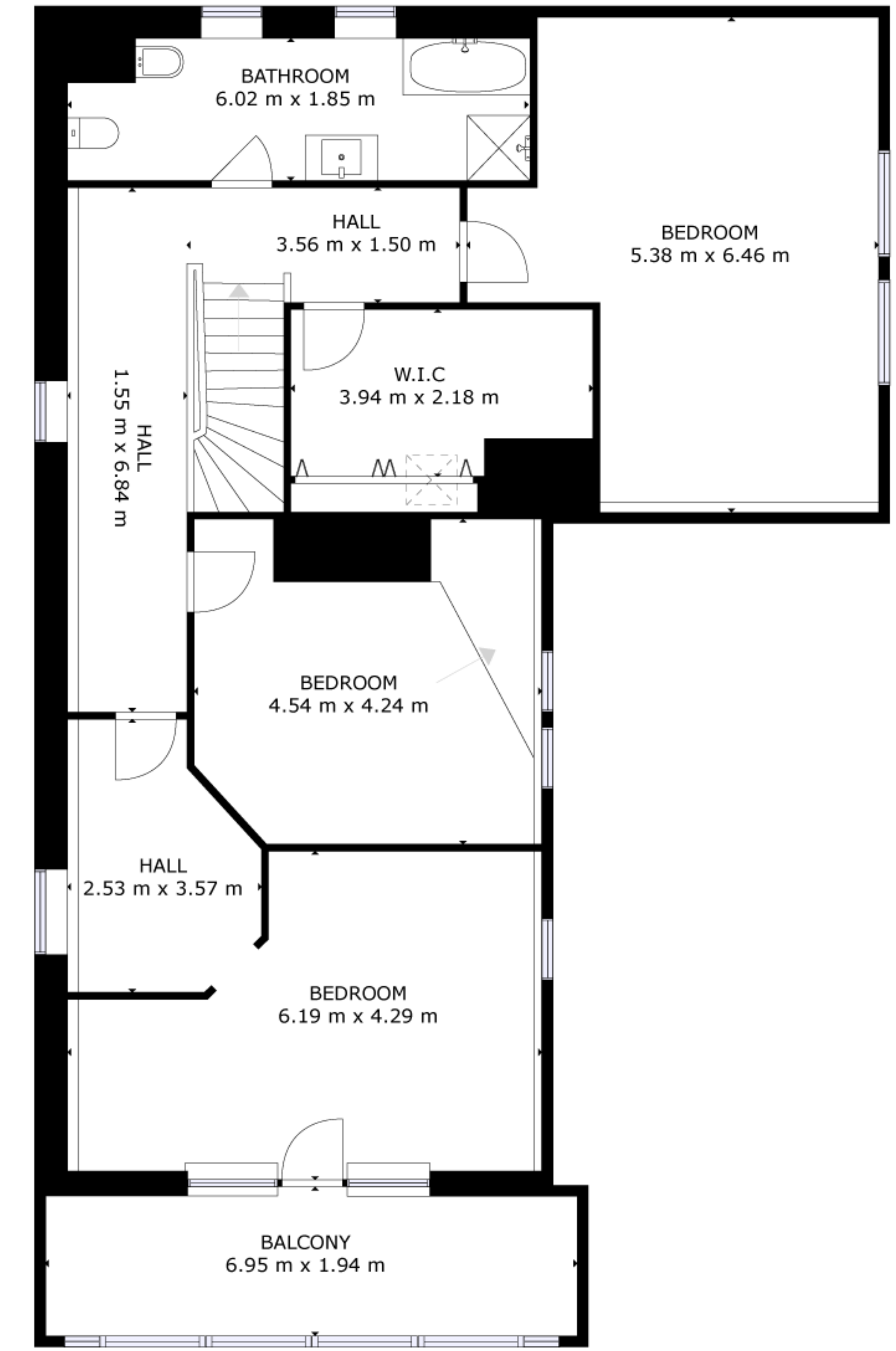
FLOOR 2
